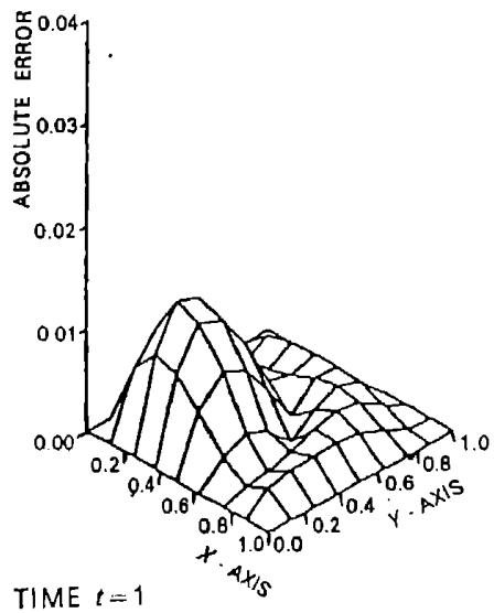
Fig. 3. |u(t) - u_{th\Delta t}(t)| , h = 1/8 , \Delta t = 1/32
