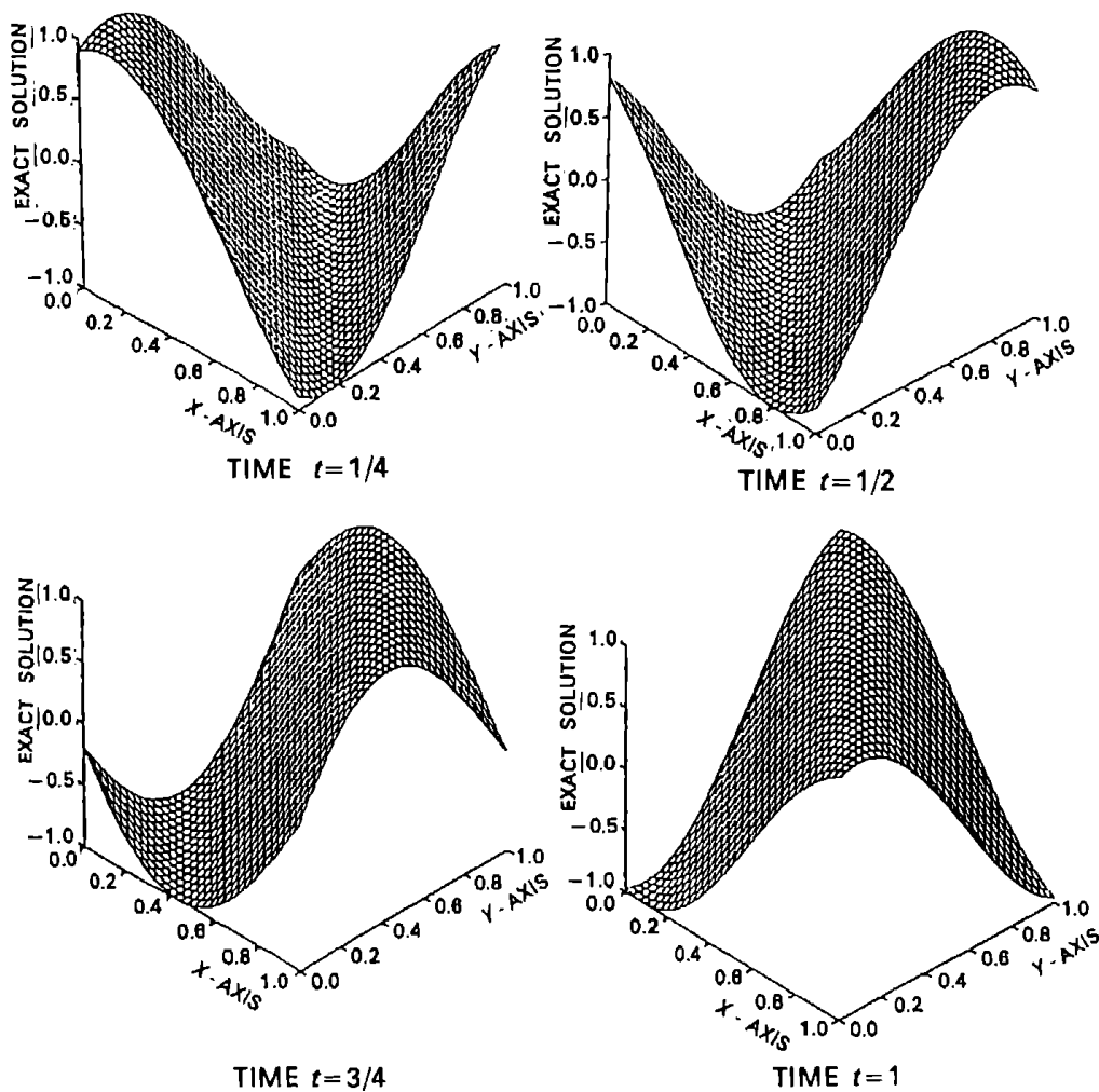
Fig. 2. The exact solution of (6.8) for t = 1/4, 1/2, 3/4 and 1
