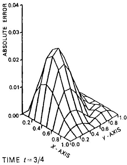
Fig. 3. |u(t) - u_{th\Delta t}(t)| , h = 1/8 , \Delta t = 1/32
