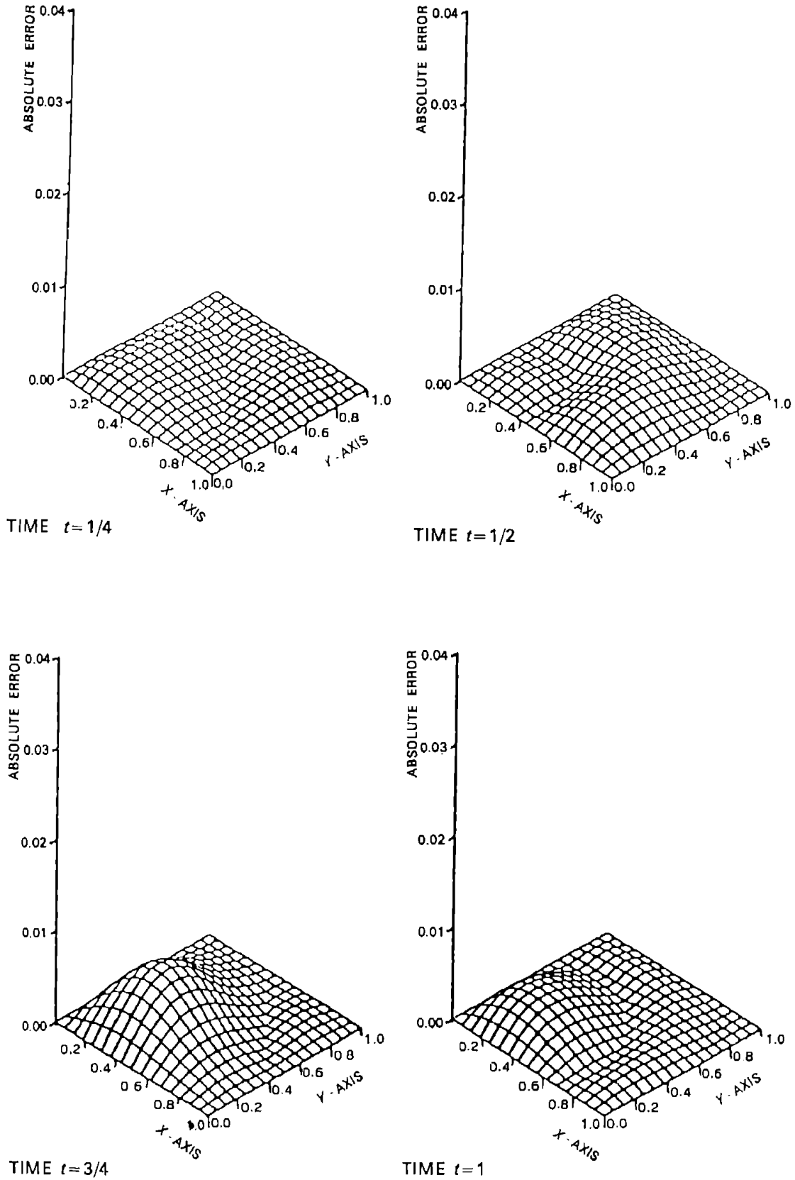
Fig. 4. |u(t) - u_{ch\Delta t}(t)| , h = 1/16 , \Delta t = 1/64
