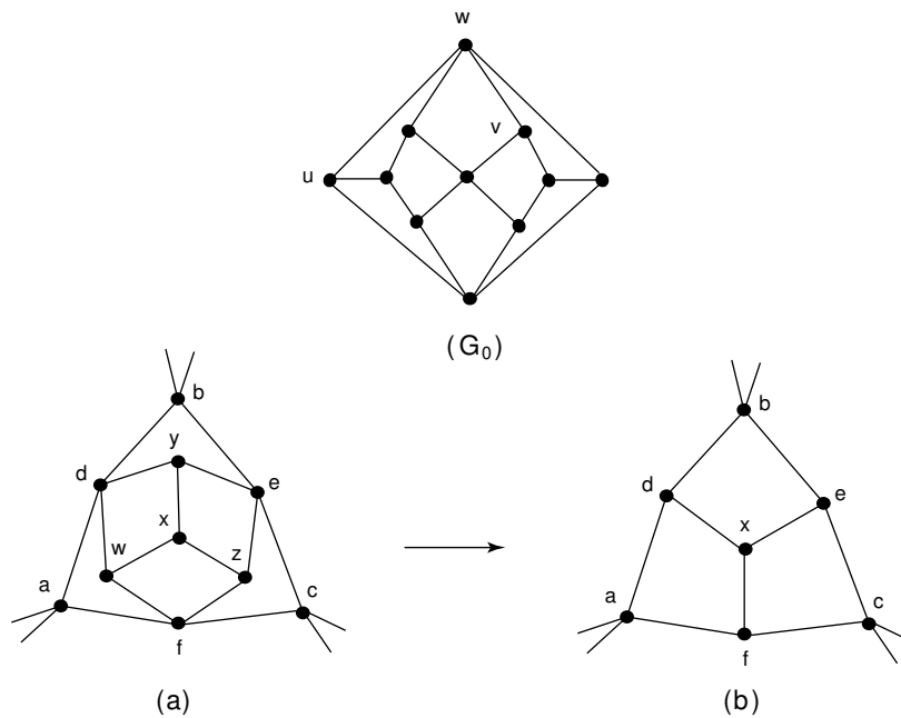
Figure 6. Graph G_0 and the method of constructing G' from G in the proofs of Lemma 3 and Theorem 1.
