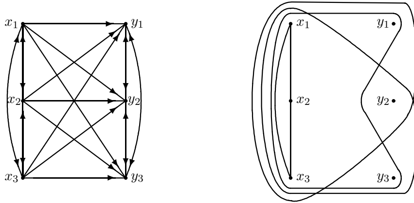
Figure 1. The digraph \tilde{D}_6 and its competition hypergraph.
