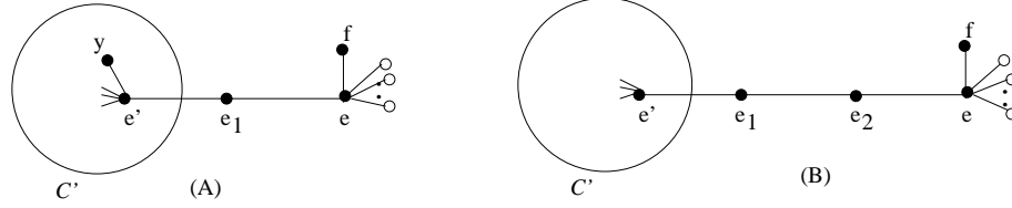
Figure 4. The extension of \sigma_{C'} to \mathcal{C} is given by: (A) \sigma_{\mathcal{C}}(e) = e_1 , \sigma_{\mathcal{C}}(e_1) = y , \sigma_{\mathcal{C}}(f') = e and \sigma_{\mathcal{C}}(f) = f , (B) (e_1, e_2, f, e) .
